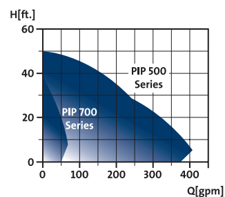
PIP500, PIP700 Small sewage and effluent pumps
