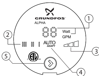
Fig. 7 Control display
