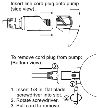
Fig. 4 Connecting and removing power plug for line cord models
