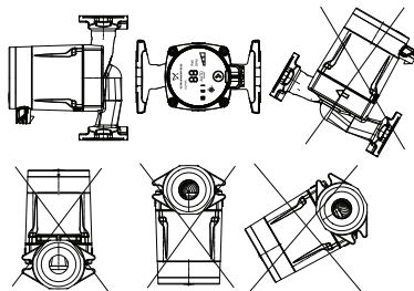
Fig. 2 Installation positions
